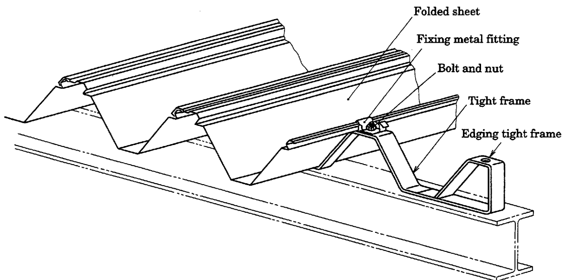
Fig. 3 Example of engagement type roof-deck
