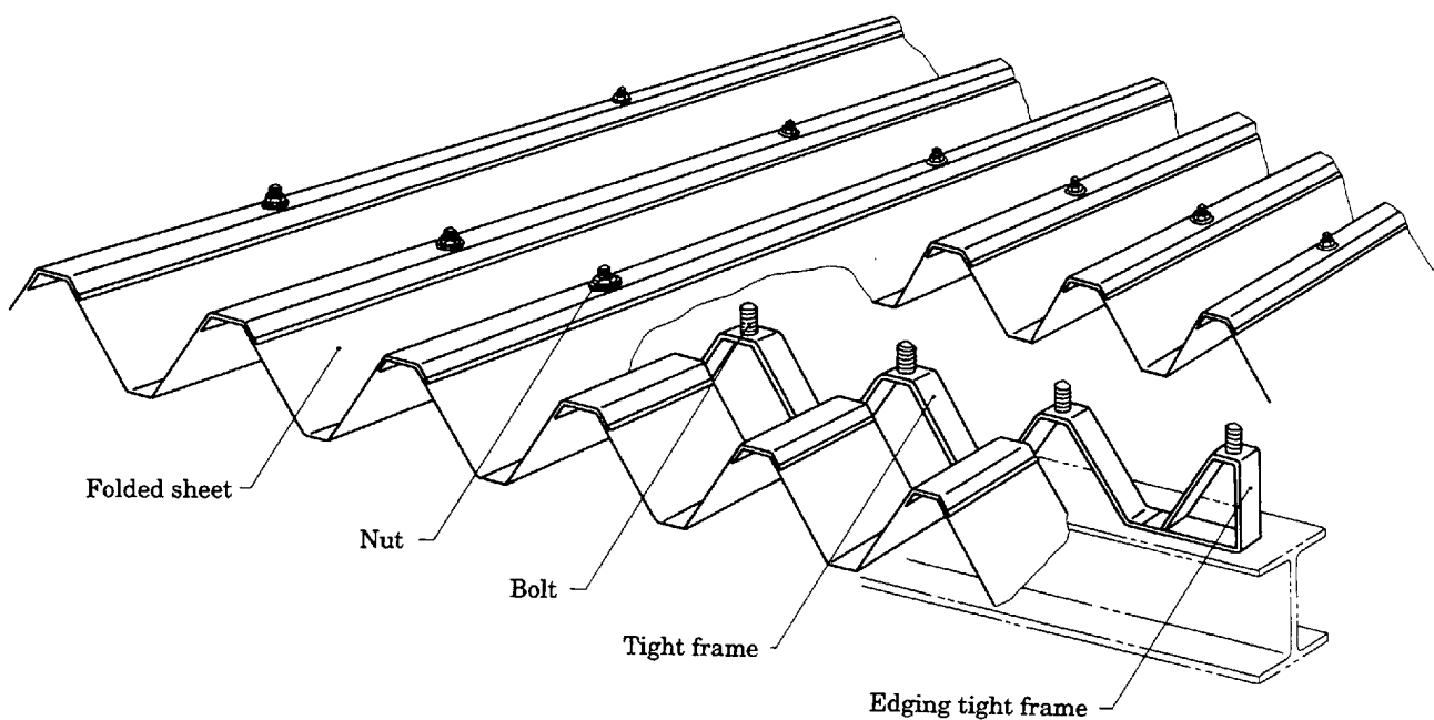
Fig. 1 Example of overlap type roof-deck
