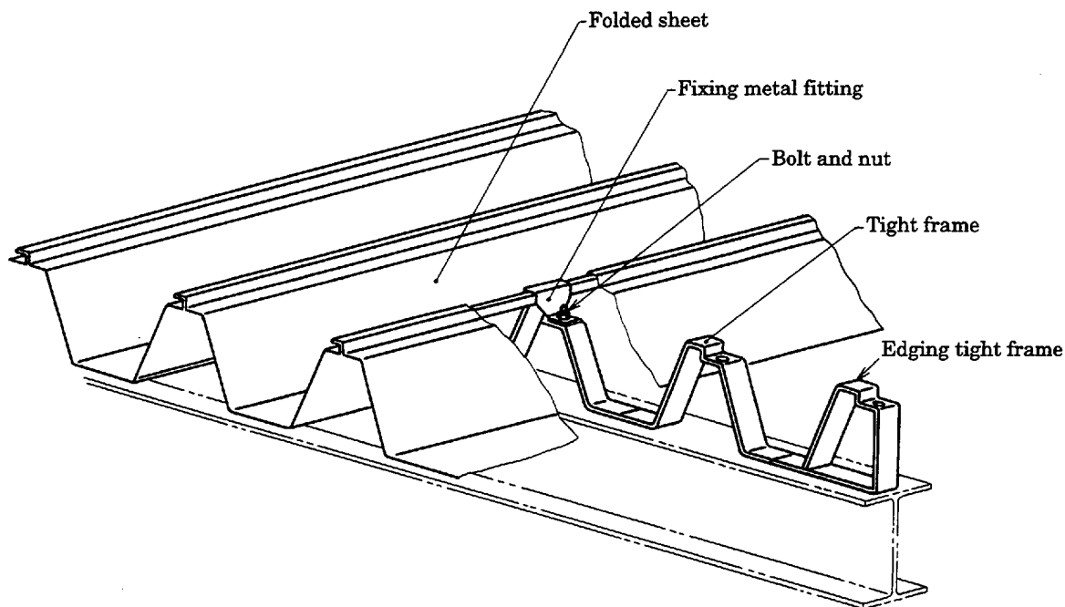
Fig. 2 Example of seam tightening type roof-deck
