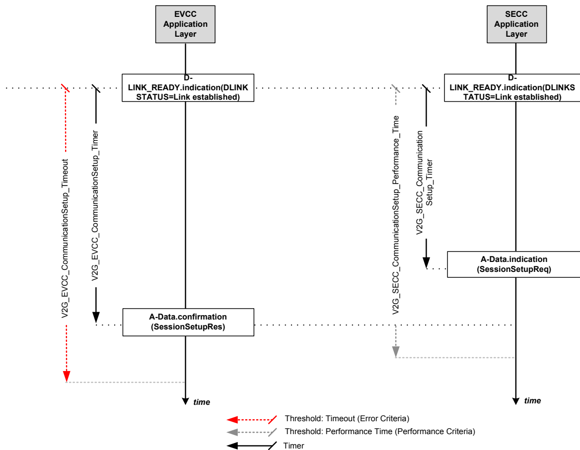
Figure 99 — CommunicationSetup timing
