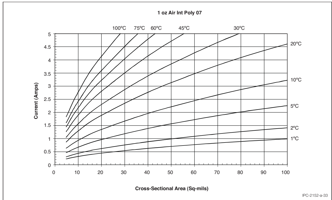
Figure A-33 1 oz. Internal Conductors (Still Air) (5 - 100 Sq-mils)
