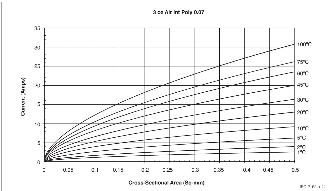
Figure A-44 3 oz. Internal Conductors (Still Air) (0 - 0.5 Sq-mm)
