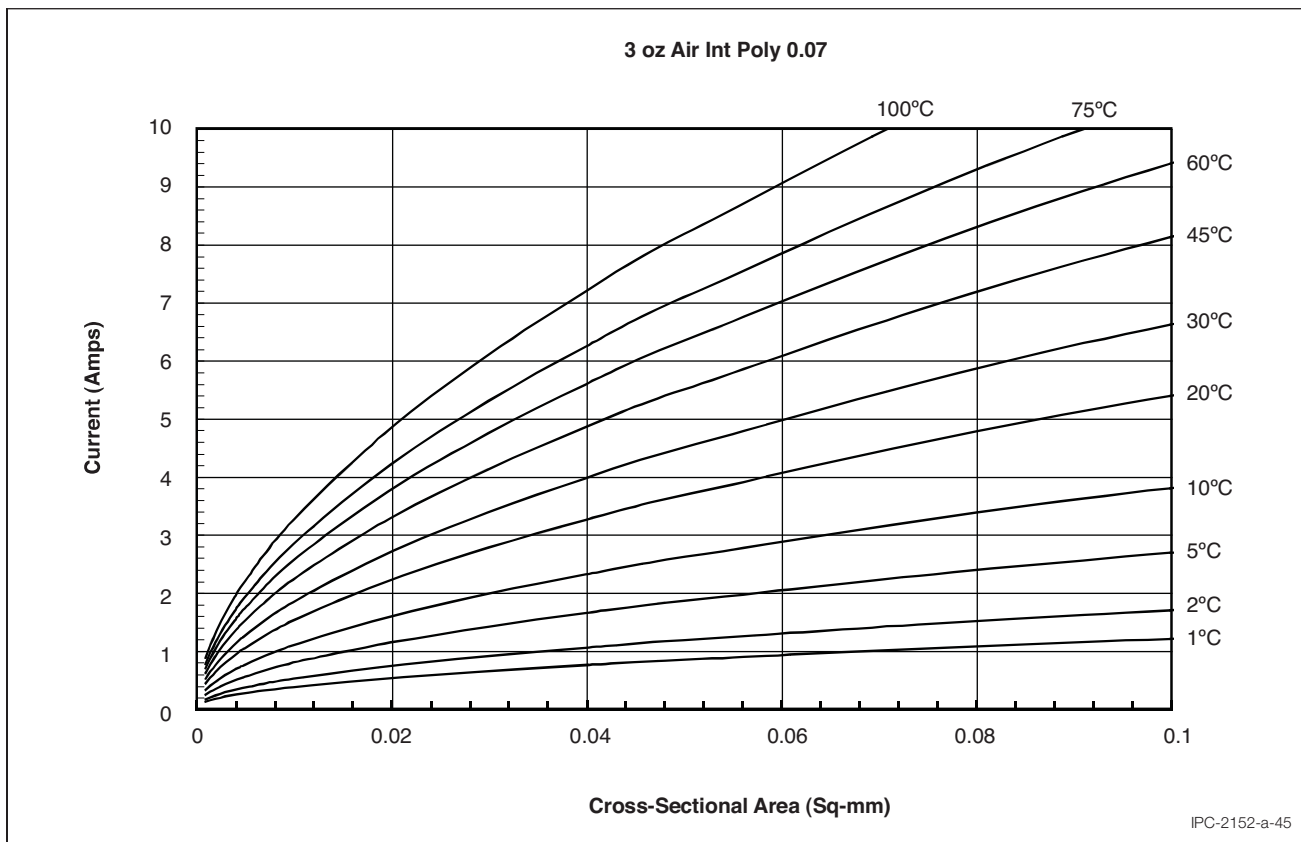
Figure A-45 3 oz. Internal Conductors (Still Air) (0 - 0.1 Sq-mm)
