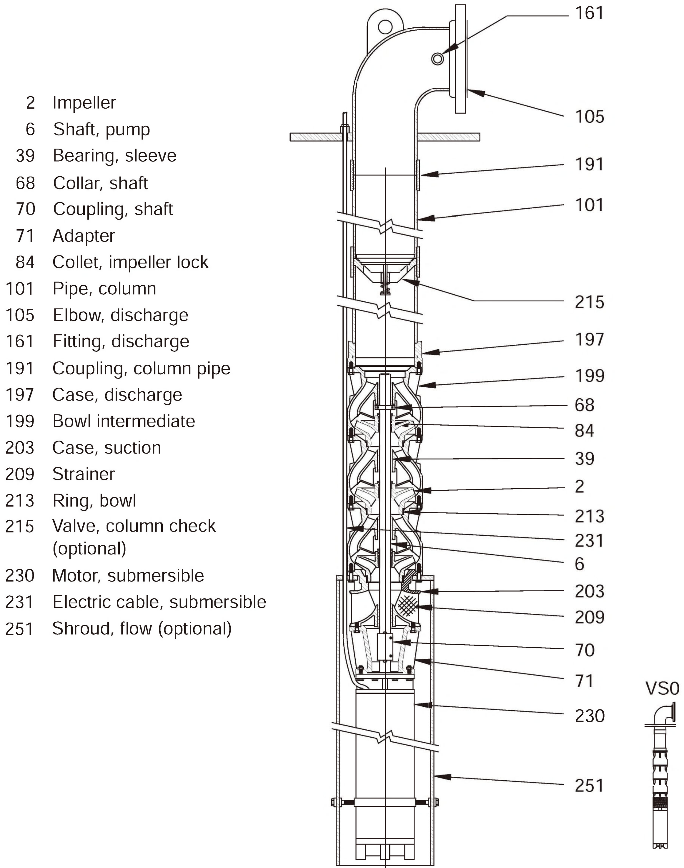
Figure 14.1.6dd — Vertically suspended – single casing – submersible pump
