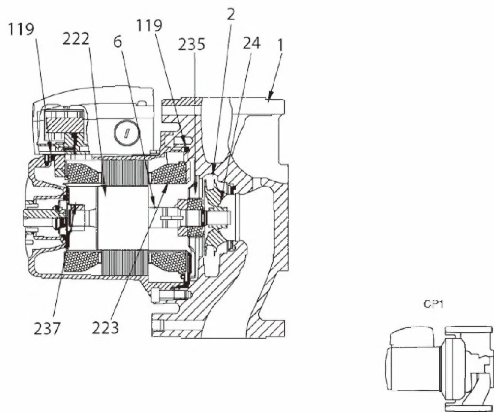
Figure 14.1.6aa — Close-coupled sealless with canned motor
