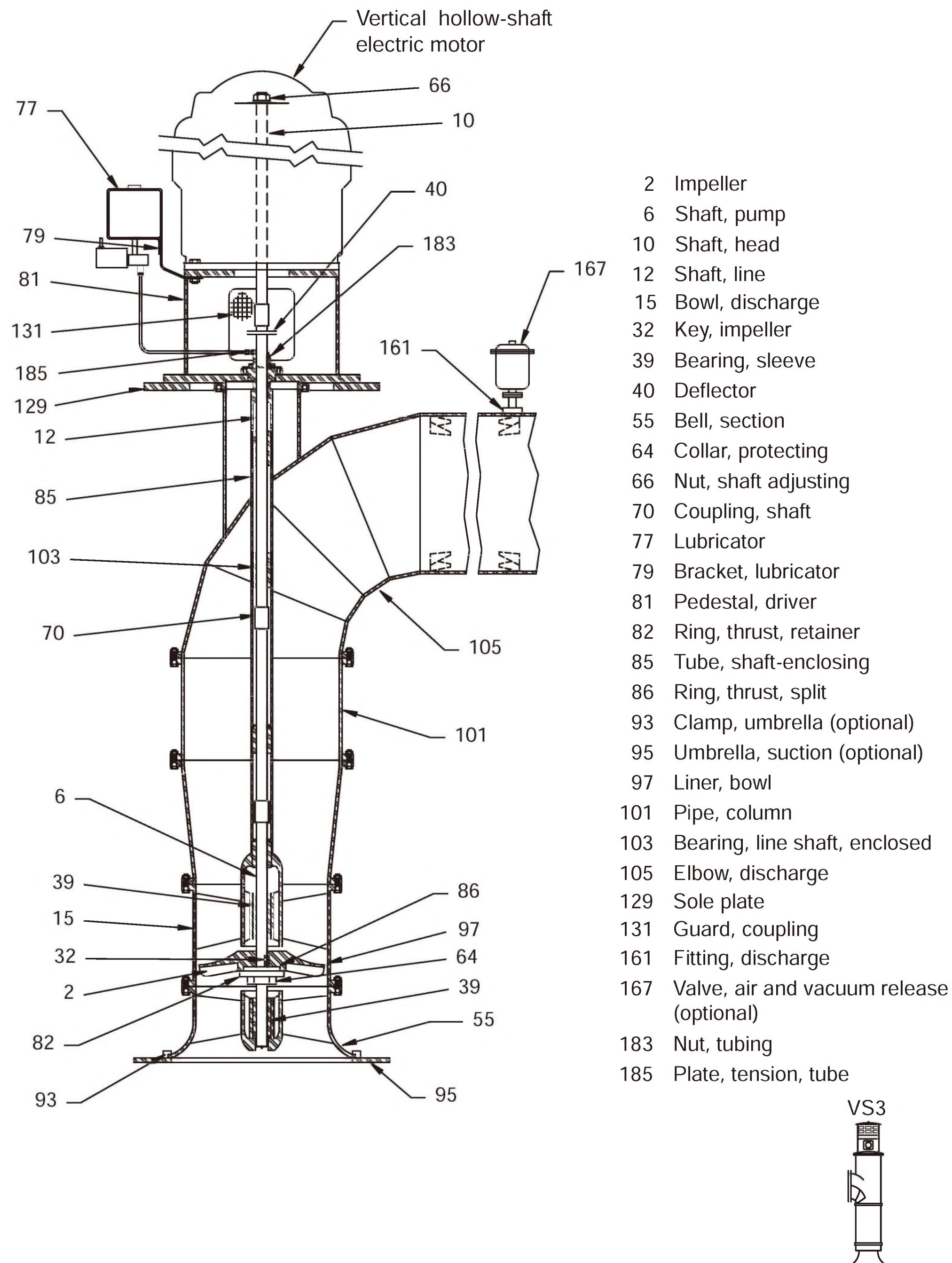
Figure 14.1.6ii — Vertically suspended – single casing – discharge through column – axial flow pump
