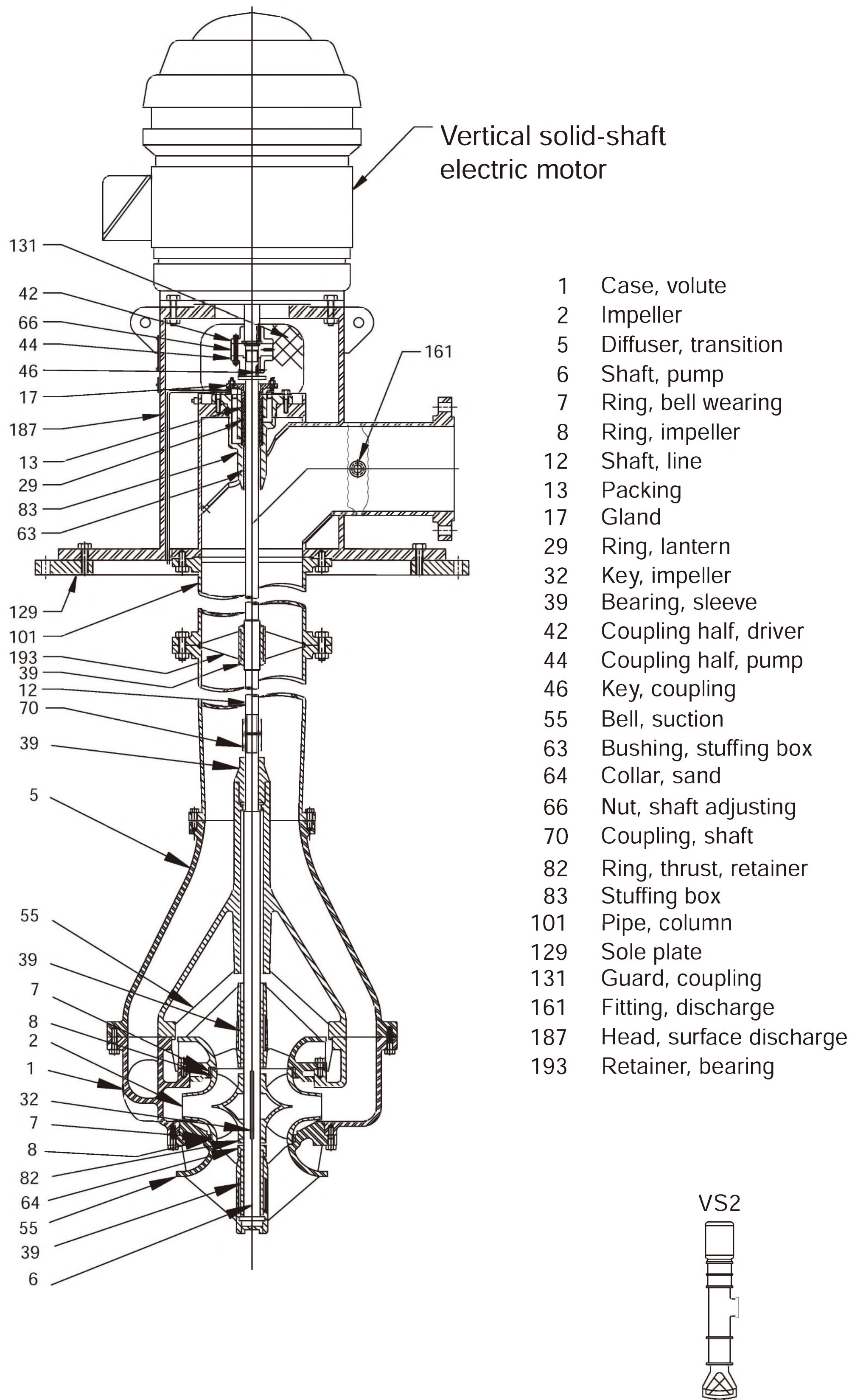
Figure 14.1.6hh — Vertically suspended – single casing – discharge through column – volute pump
