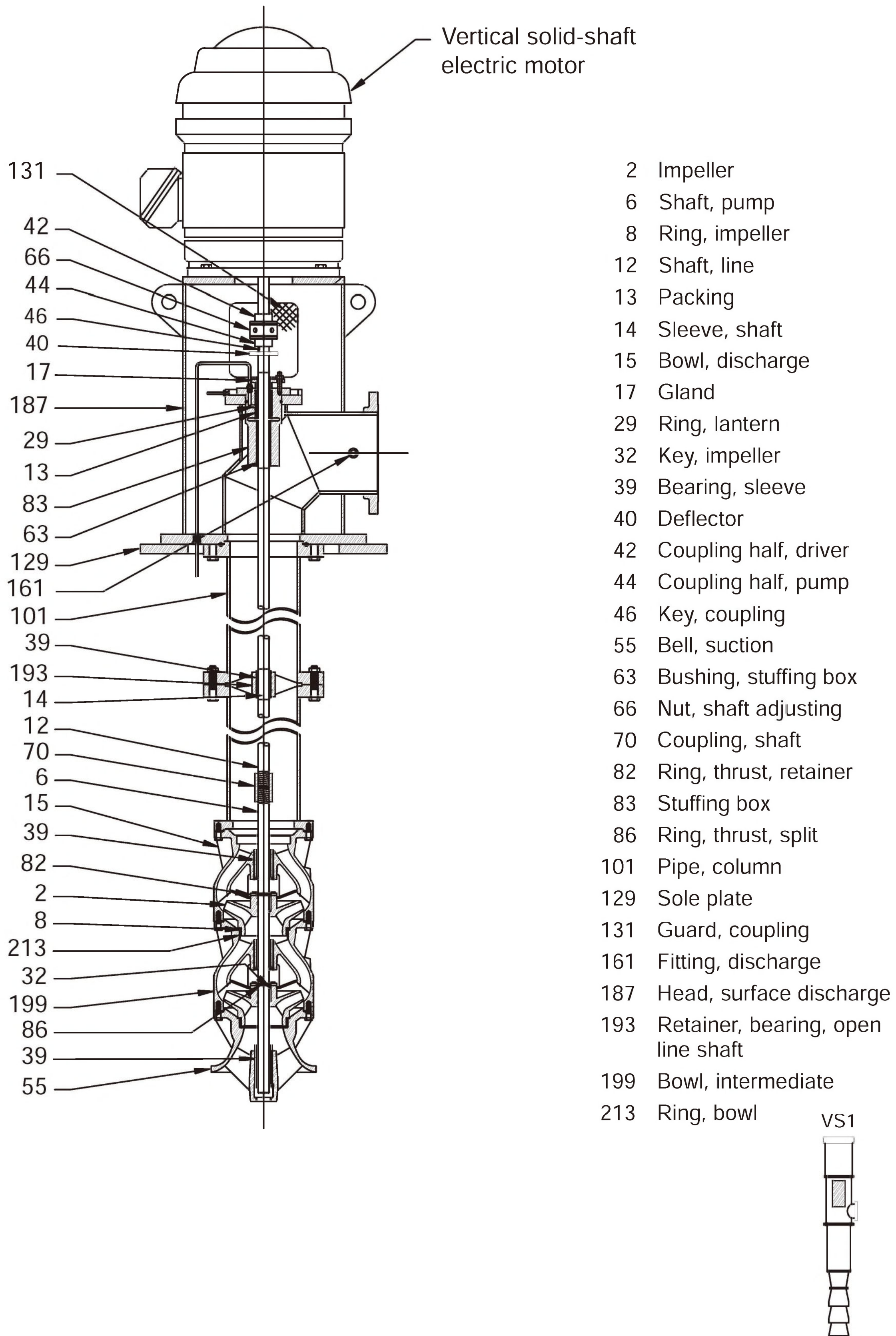
Figure 14.1.6ff — Vertically suspended – single casing – discharge through column – short-set pump
