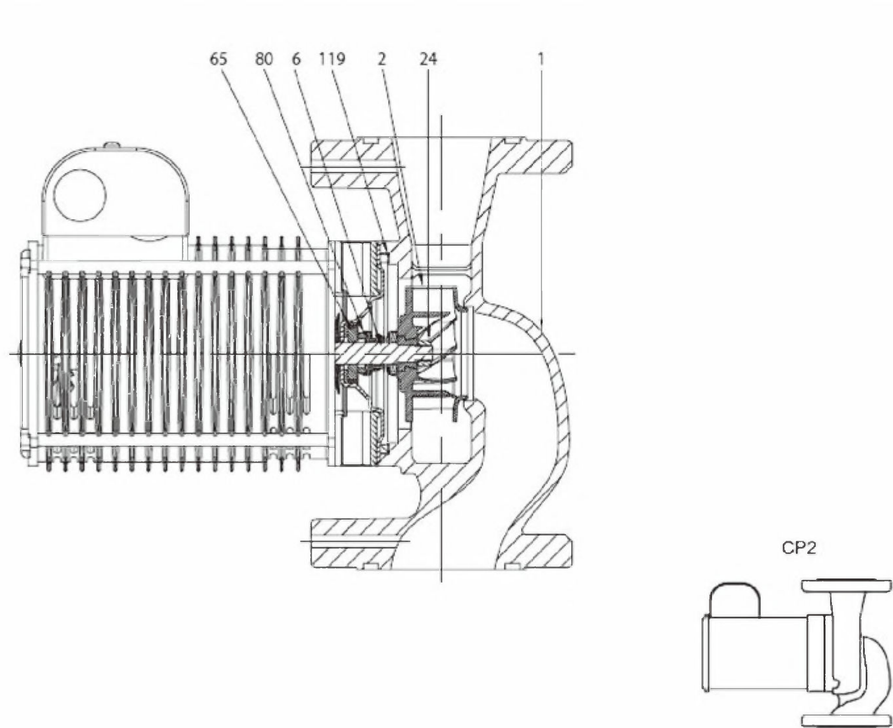
Figure 14.1.6bb — Close-coupled horizontal in-line
