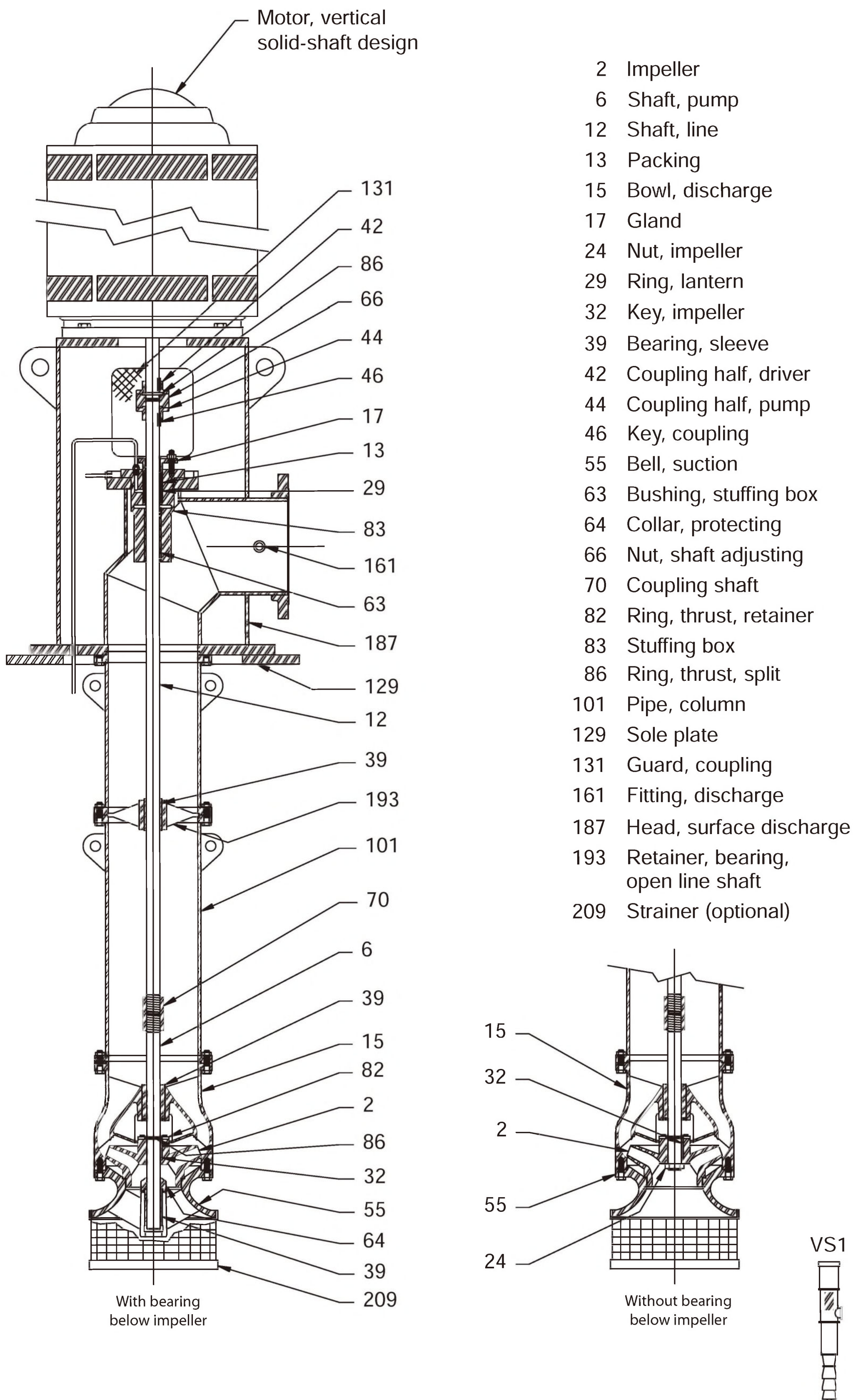
Figure 14.1.6gg — Vertically suspended – single casing – discharge through column – short-set - mixed flow pump
