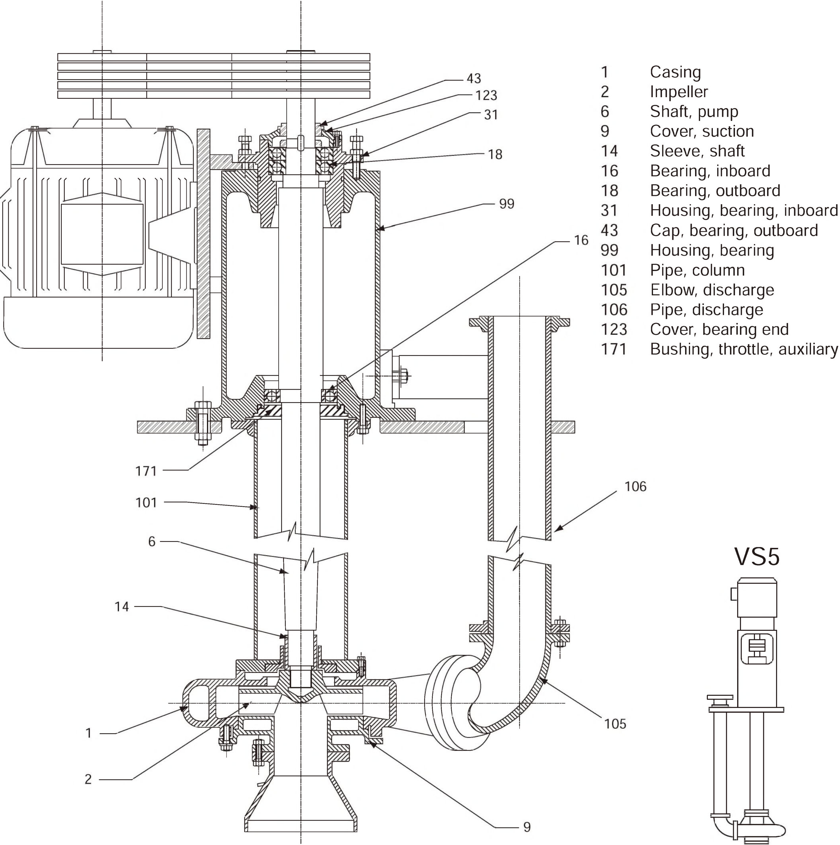
Figure 14.1.6kk — Vertically suspended – single casing – separate discharge – cantilever pump
