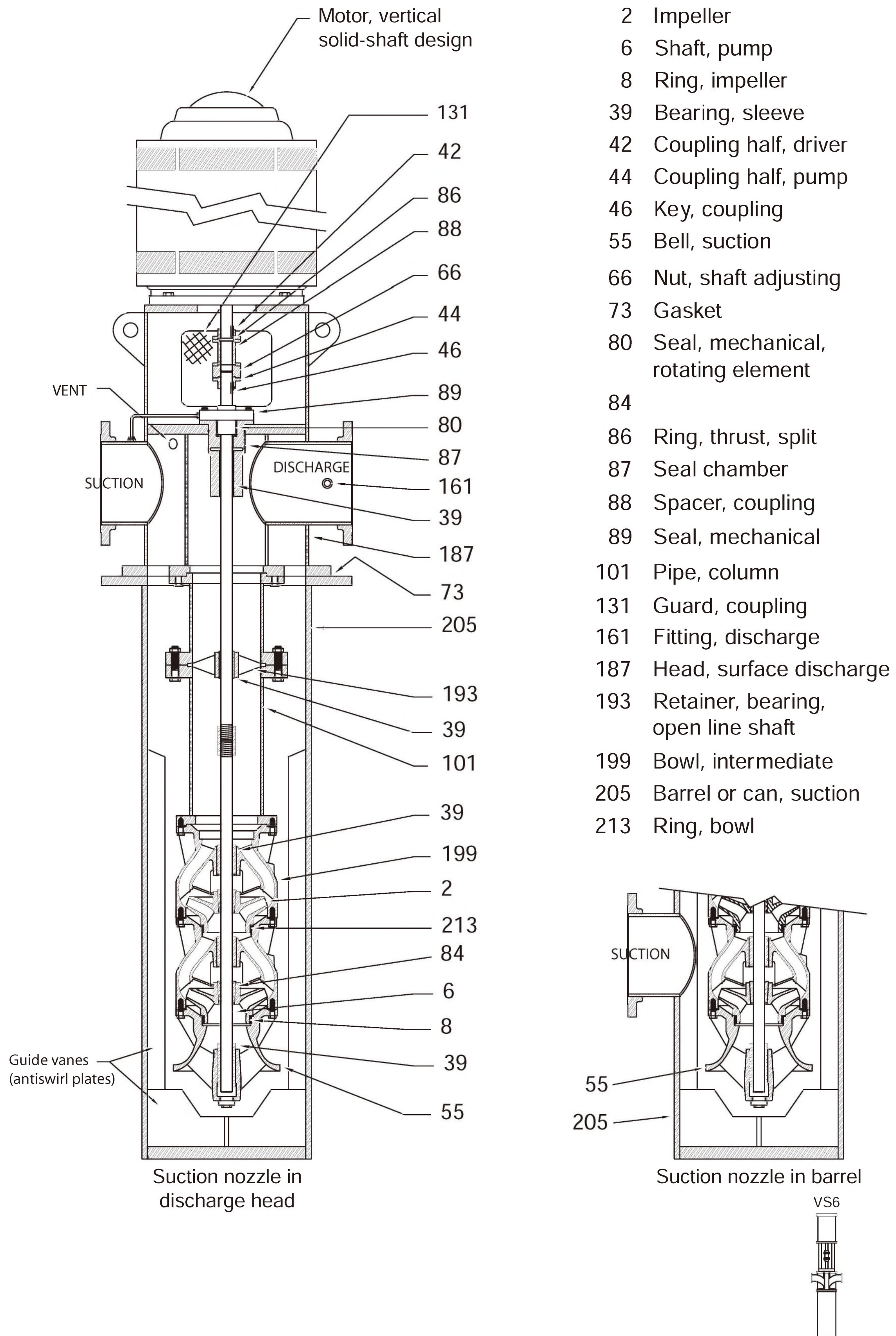
Figure 14.1.6II — Vertically suspended – double casing – diffuser pump
