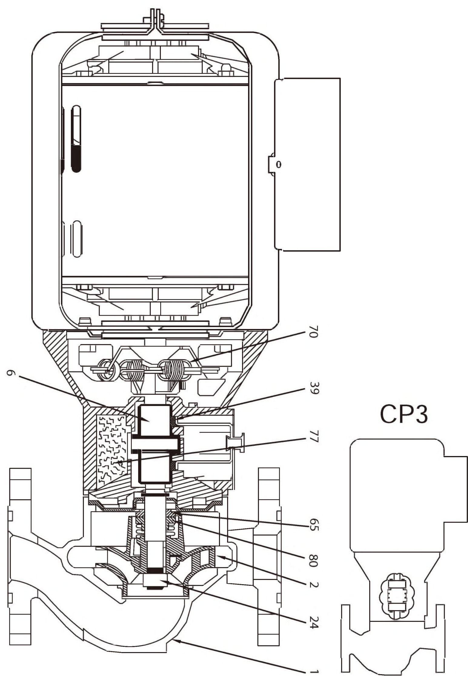
Figure 14.1.6cc — Flexibly coupled horizontal in-line
