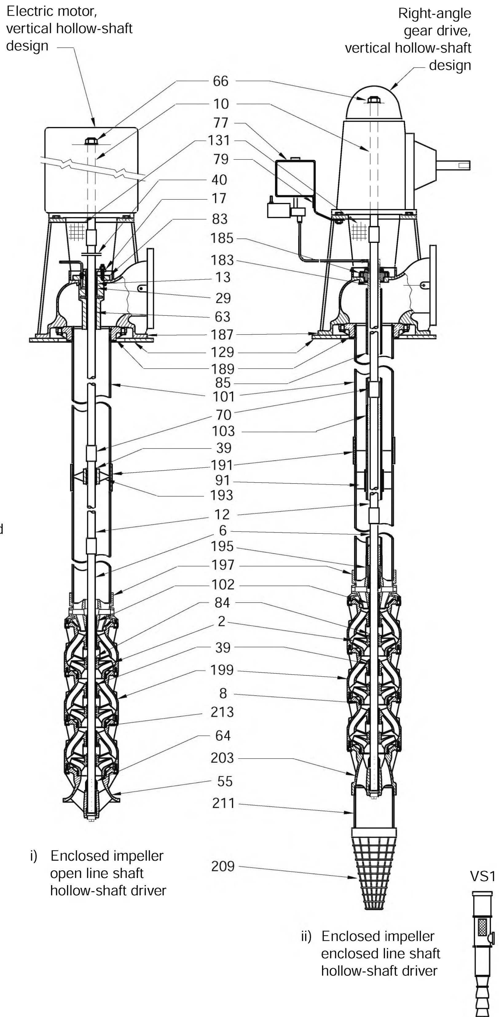
Figure 14.1.6ee — Vertically suspended – single casing – discharge through column – deep-well (set) pumps
