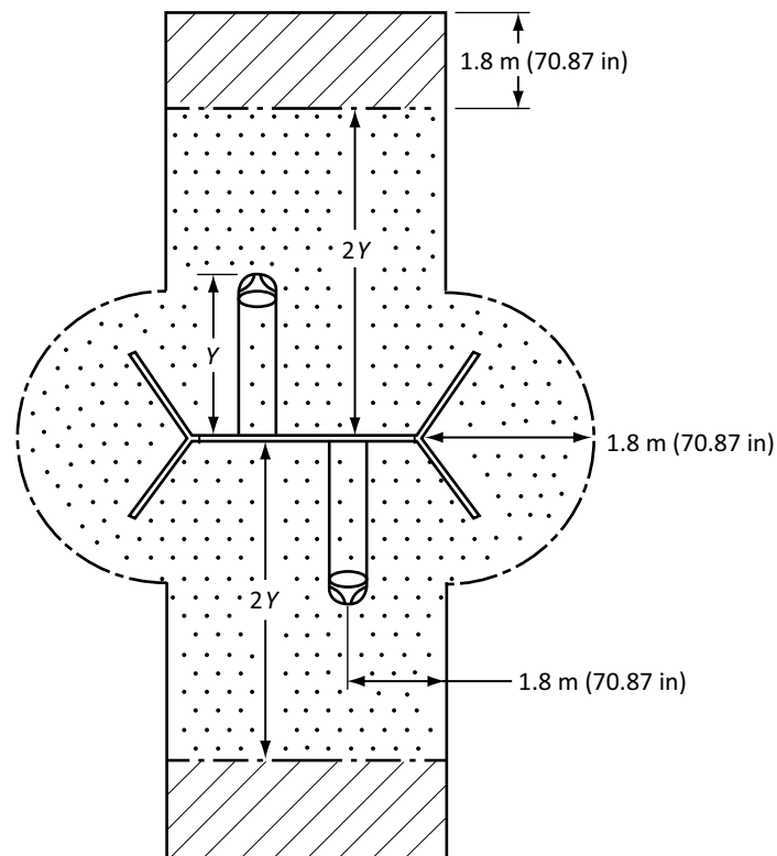
Figure 28 Protective surfacing and no-encroachment zones for single axis swings with enclosed seats
