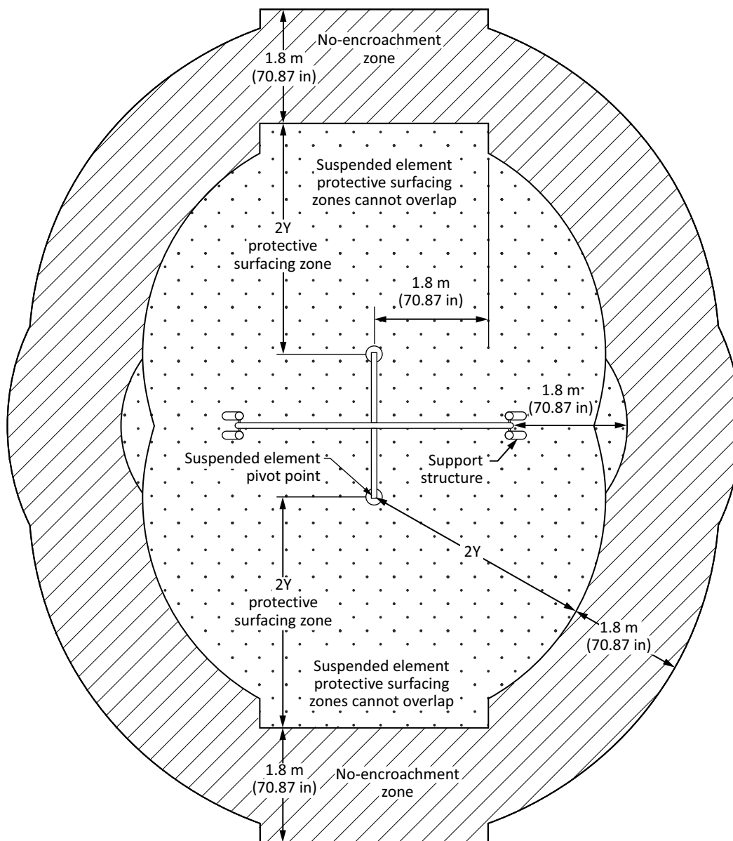
Figure 30 Protective surfacing and no-encroachment zones for combination swings (See Clause 14.4.3. )
