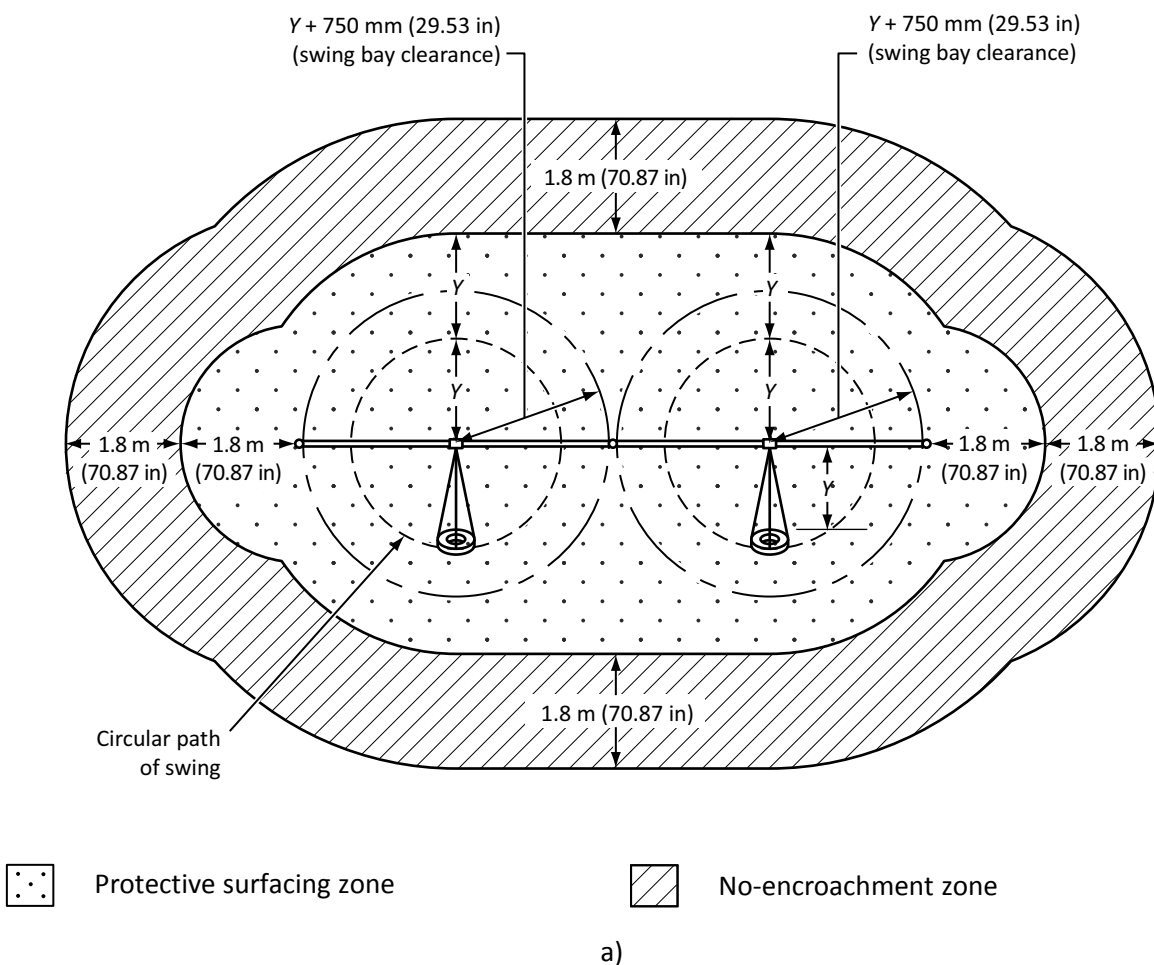
Figure 29 Protective surfacing and no-encroachment zones for rotating swings (See Clauses 14.4.2.1 to 14.4.2.4. )
