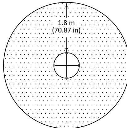
Figure 26 Protective surfacing zone for rotating equipment (See Clauses 14.3.1 and 14.3.2 .)
