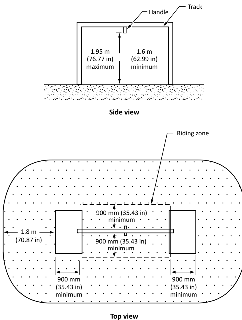
Figure 34 Details of a track ride (See Clauses 14.7 , 15.13.2.1 , 15.13.3.1 , and 15.13.4.1 .)
