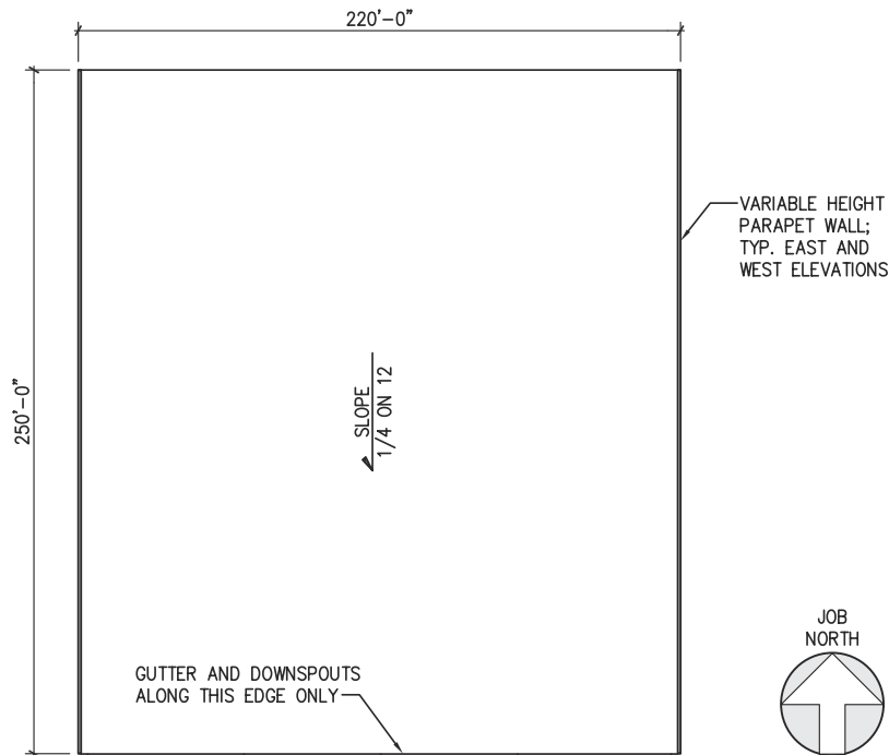
Fig. G8-5. Plan view of monoslope roof for Example 8-1
